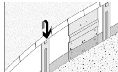
STEP 6 - Place edge onto pegs and use rubber mallet to hammer edge on so peg locks in. Work down the line.
