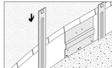
STEP 5 - With line just right, hammer all pegs adjacent edge (three per length) leaving them just above finishing height.
