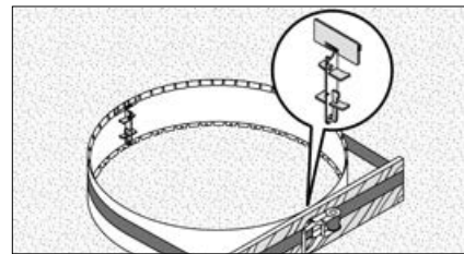
STEP 4 - When the edge end joint flanges align perfectly, use joining set to lock together.
